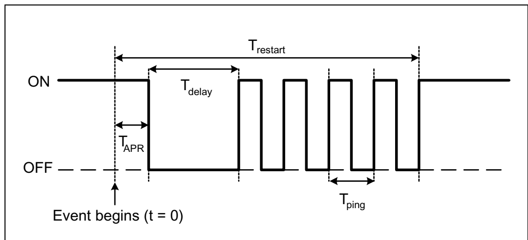
FIGURE 2. Example Timing Diagram for an APR Response
