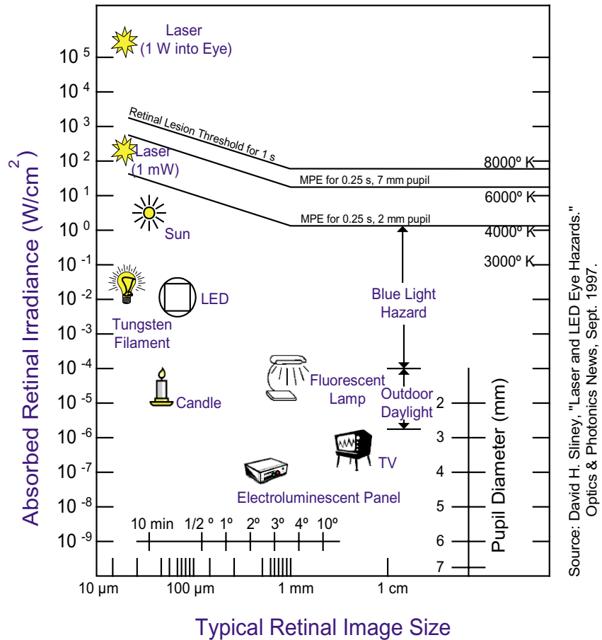
FIGURE 1. Retinal irradiance for a variety of sources. The retinal image area influences the hazard as does the source radiance.
